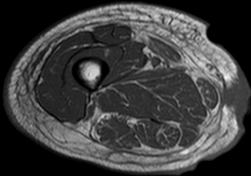
T1WI
