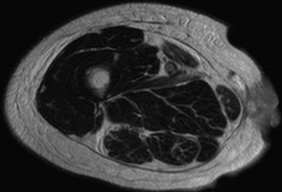
T2WI
