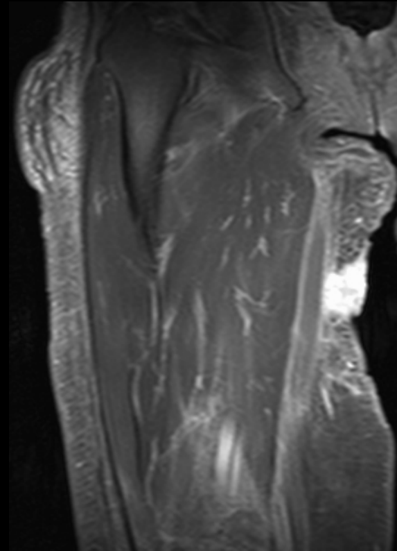
coronal
