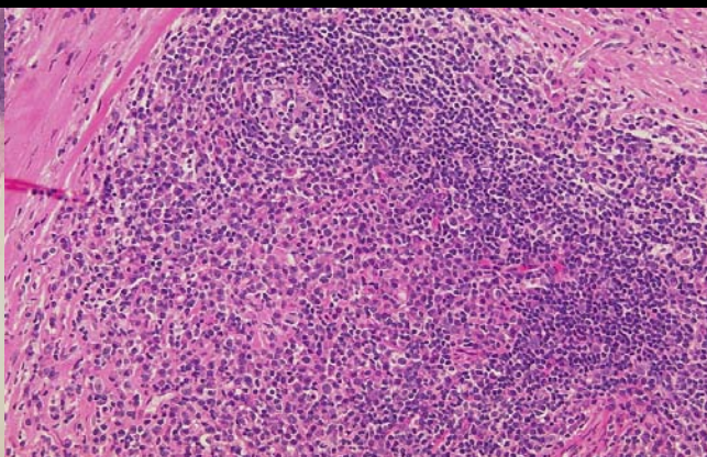
HE 20x
