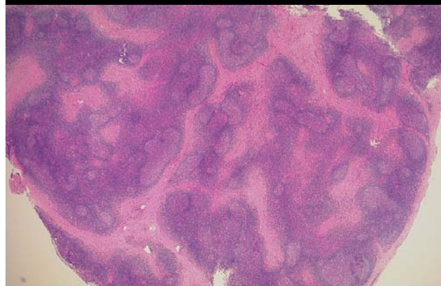
HE 2x
