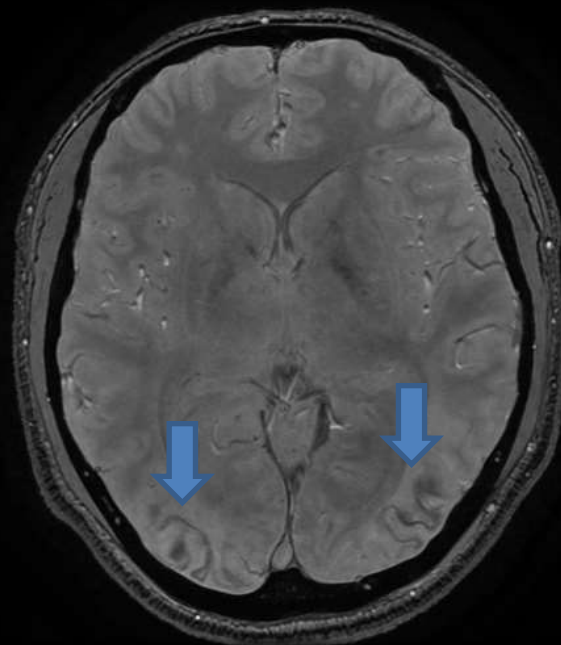
SWI (SWAN)
